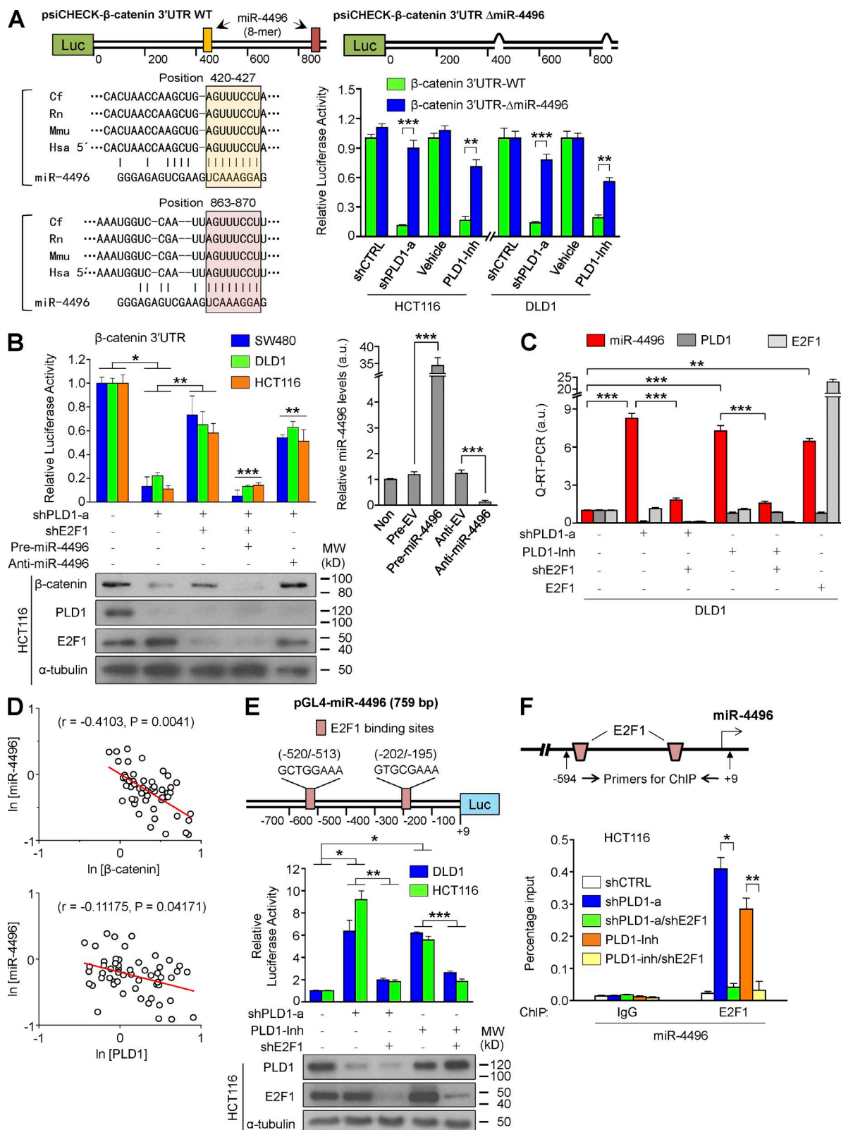
Figure 7. PLD1 inhibition down-regulates \beta -catenin expression through E2F1-induced miR-4496 up-regulation. (A) Schematic representation of luciferase constructs of \beta -catenin 3' UTR. Luciferase vectors (psiCHECK) were inserted with full-length \beta -catenin 3' UTR (930 bp). \Delta miR-4496 (914 bp) were generated by deletions of highly conserved and predicted binding sites for the seed sequences of the miR. Effect of depletion or inhibition of PLD1 on the luciferase activity of \beta -catenin 3' UTR reporters. A Student's t test was used. The pink and peach boxes represent conserved seed pairing. (B) Effect
