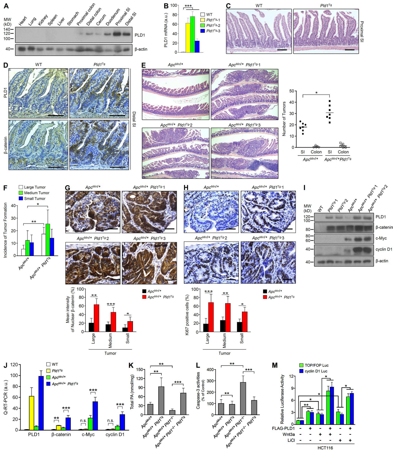
Figure 5. IEC-specific PLD1 overexpression accelerates tumorigenesis in Apc Min/+ mice. (A) PLD1 expression in various tissues from IEC-specific PLD1 Tg mice. Results are representative of at least four independent experiments. (B) q-RT-PCR analysis in SI from WT and Pld1 Tg mice. n = 5 per group. (C and D) WT ( n = 5) and Pld1 Tg ( n = 6) mice were sacrificed at 12 weeks for histology analysis. H&E staining (C) and IHC for PLD1 and \beta -catenin (D). (E) The histology of representative tumors (left) and incidence of tumor formation (right; n = 7 per group). (B–D) A Student's t test was used. (F) Size distribution of polyps in the SI of the indicated mice. n = 7 per group. ANOVA F-test was used. (G and H) IHC for \beta -catenin (G) and Ki67 (H). Representative images were selected from at least three different fields. The expressions of nuclear \beta -catenin (G) and Ki67 (H) were quantified in size distribution of polyps. n = 5 per group; 10 tumors per mouse.
