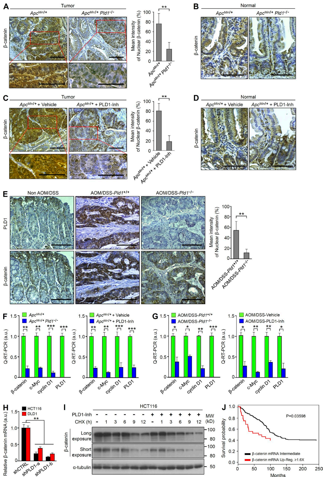
Figure 4. PLD1 inactivation down-regulates expression of β-catenin. (A–D) IHC for β-catenin in tumor tissues (A) and normal mucosa (B) of Apc Min/+ and Apc Min/+ Pld1 -/- mice and in tumor tissues (C) and normal mucosa (D) of Apc Min/+ /vehicle and Apc Min/+ /PLD1-Inh mice. The nuclear β-catenin in the tumor was quantified (A and C, right). n = 21 per group; five tumors per mouse. (E) IHC for PLD1 (top) and β-catenin (bottom) in normal colon mucosa of non-AOM/
